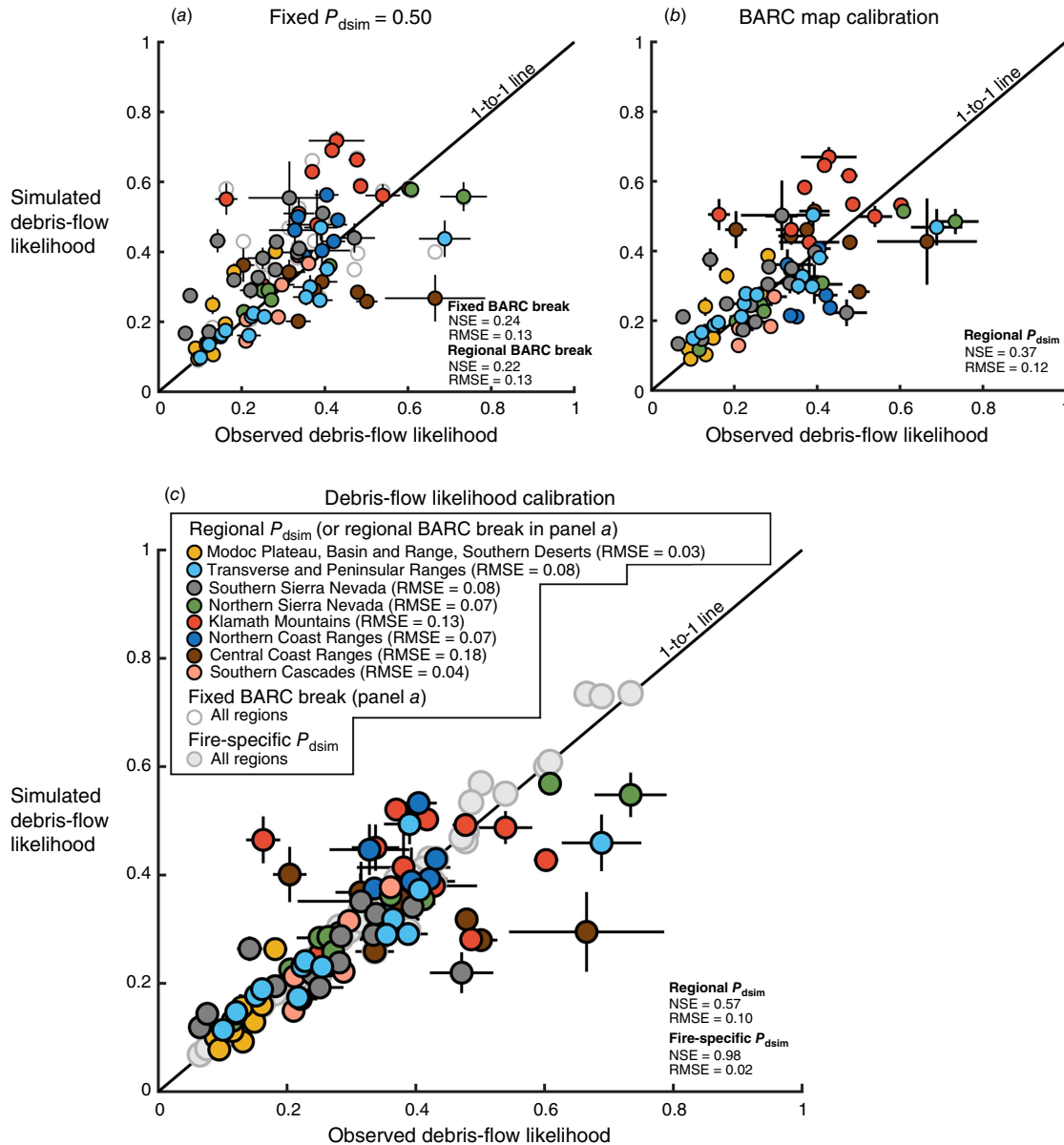
Fig. 7. Comparison of fire-wide mean debris-flow likelihood for fixed P_{dsim} = 0.50 (a) and calibration to best match to percent moderate-high burn severity (i.e. Burned Area Reflectance Classification (BARC) map calibration) (b), and lowest Root Mean Square Error (RMSE) for observed and simulated debris-flow likelihood (i.e. DFL calibration) (c). Uncertainty bars show two standard errors of the mean for the basins inside the respective fire perimeter. The uncertainty bars indicate the relative width of the distributions for the simulated and observed debris-flow likelihood for a single fire (since the sample size for simulated and observed debris-flow likelihood match for the same fire). Results and statistics are for simulated and observed debris-flow likelihood for basin dNBR_{obs} > unburned -low BARC break ( T_{low} ). Abbreviations: dNBR, differenced Normalized Burn Ratio; NSE, Nash-Sutcliffe Efficiency.
